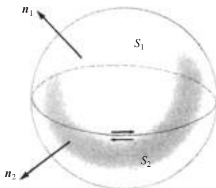
FIGURE 12.17 Extension of Stokes' theorem to a sphere.
