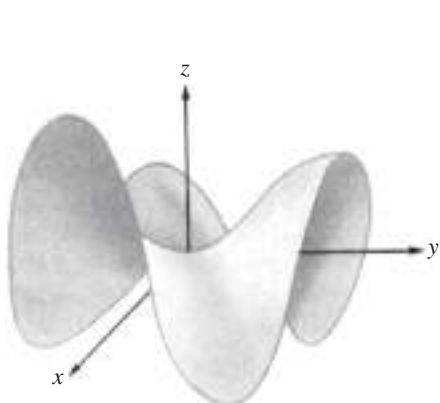
(a) z = x^3 - 3xy^2 .
