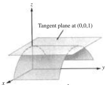
(a) z = 1 - x^2
