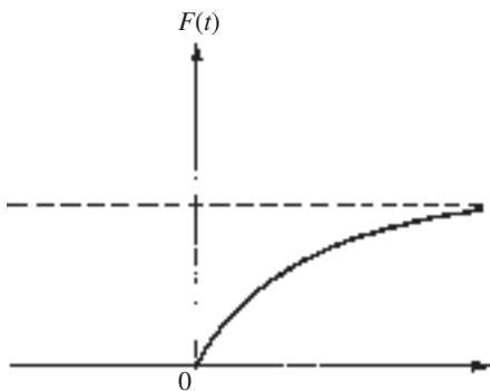
(a) The distribution function F .
