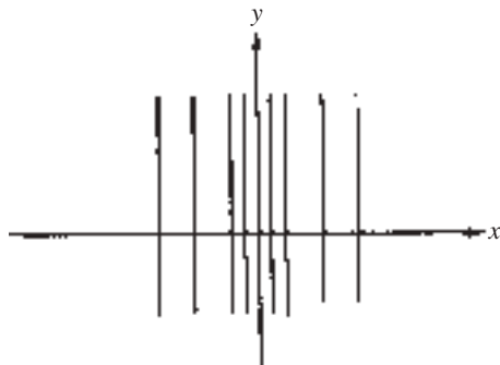
(b) Level curves: 1 - x^2 = c
