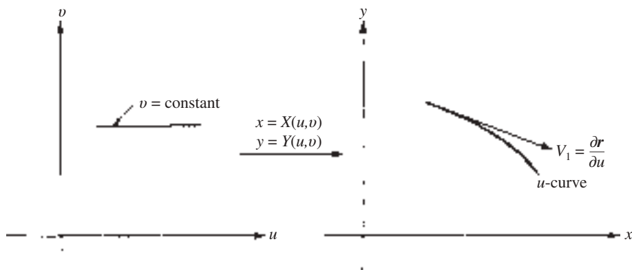
FIGURE 11.24 A u -curve and a corresponding velocity vector.
