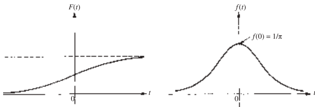
(a) The distribution function F .
