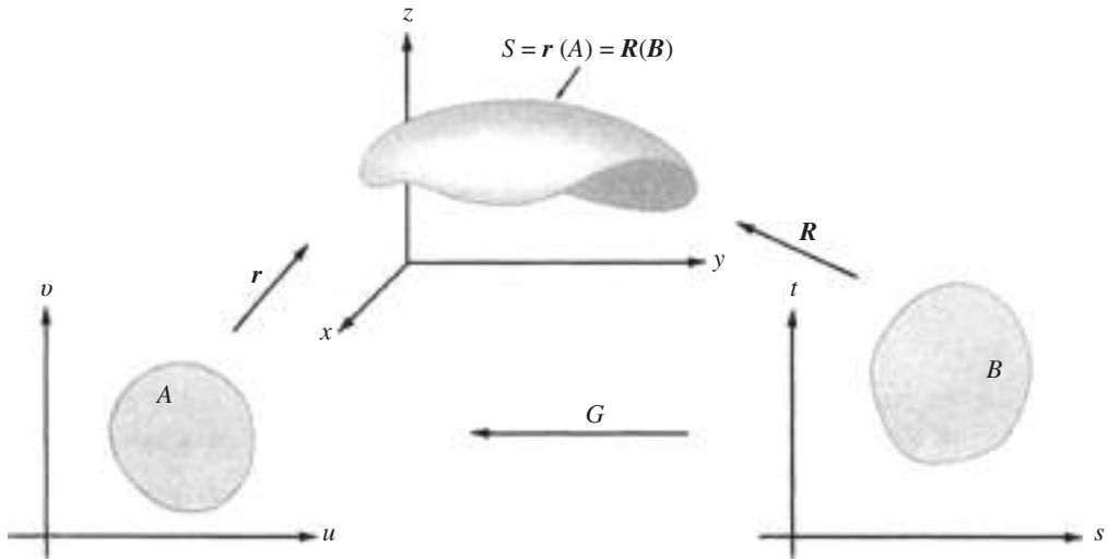
FIGURE 12.11 Two parametric representations of the same surface.
