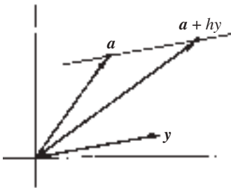
FIGURE 8.3 The point \mathbf{a} + h\mathbf{y} lies on the line through \mathbf{a} parallel to \mathbf{y} .
