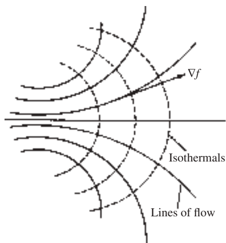
FIGURE 8.6 The dotted curves are isothermals: f(x, y) = c . The gradient vector \nabla f points in the direction of the lines of flow.
