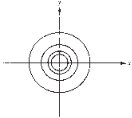
(b) Level curves: x^2 + y^2 = c
