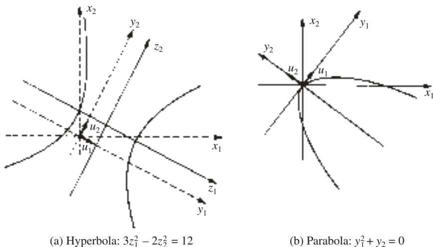
FIGURE 5.3 The curves in Examples 2 and 3.
