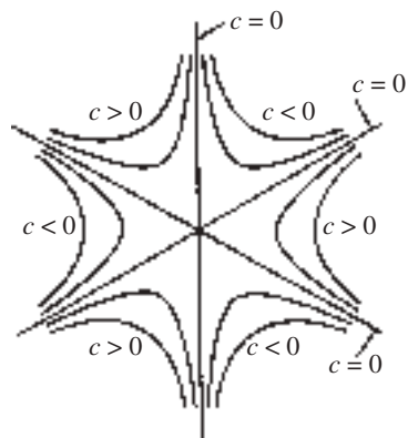
(b) Level curves: x^3 - 3xy^2 = c .
