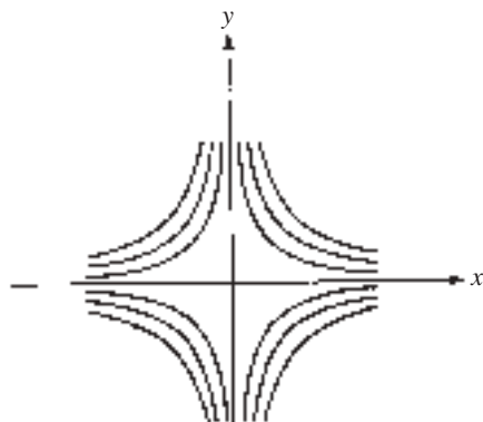
FIGURE 9.5 Example 4. Saddle point at the origin.
