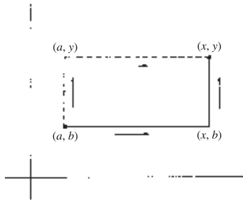
FIGURE 10.5 Two polygonal paths from (a, b) to (x, y) .
