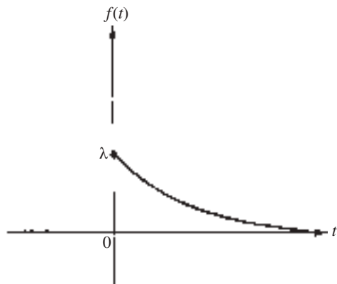
(b) The density function f .
