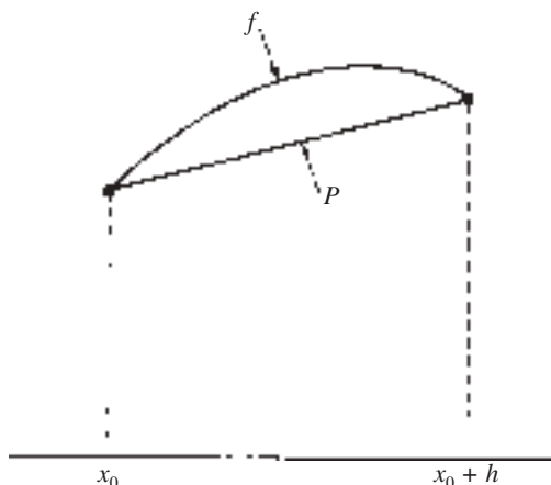
FIGURE 15.1 Linear interpolation.
