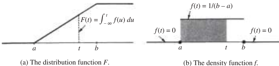
FIGURE 14.6 A uniform distribution over an interval [a, b] and the corresponding density function.
